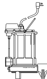
Model 257 VMF (U.S. Patent #5324171) VMF switch, magnetically operated vertical float – operates in a 10" diameter sump.
